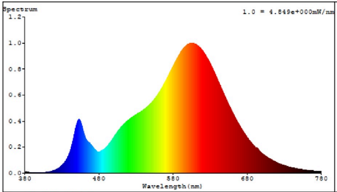
Spectral Distribution
